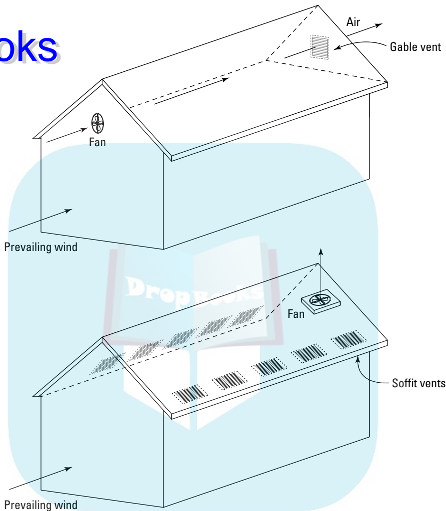
Figure 13-8: Attic vent fans may blow air upward or horizontally through the attic.
